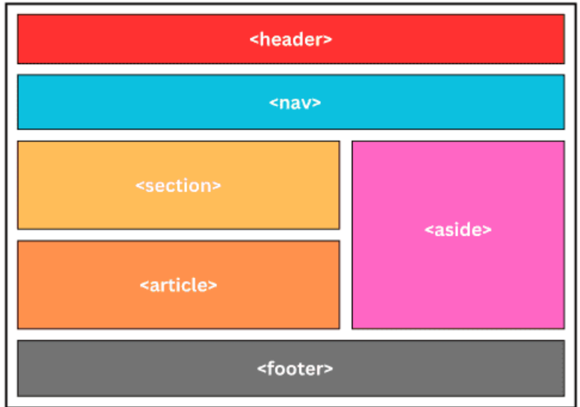
Fig: HTML Webpage Layout
